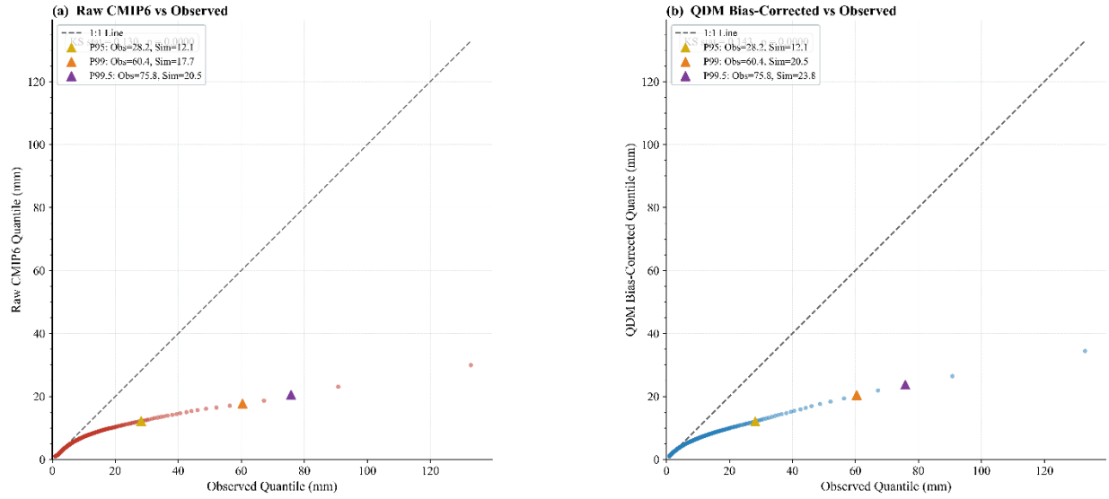
Quantile-Quantile Plot — Wet-Day Rainfall | Prachuap Khiri Khan Triangles: P95, P99, P99.5 quantile pairs | KS test statistic shown
